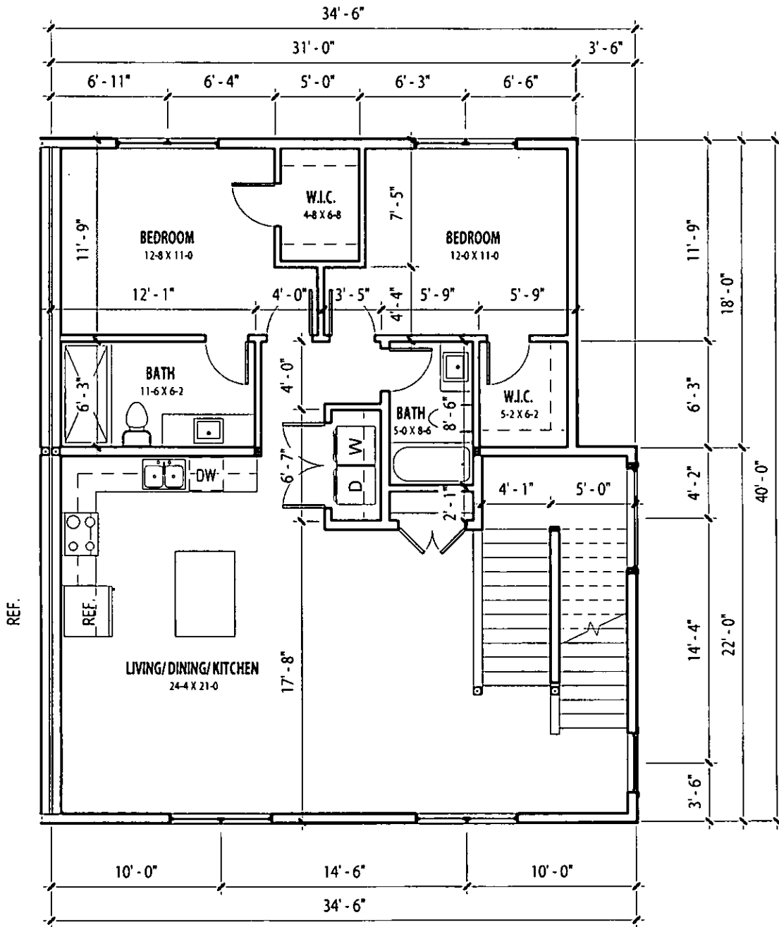
1 2ND FLOOR PLAN 1/8" = 1'-0"
