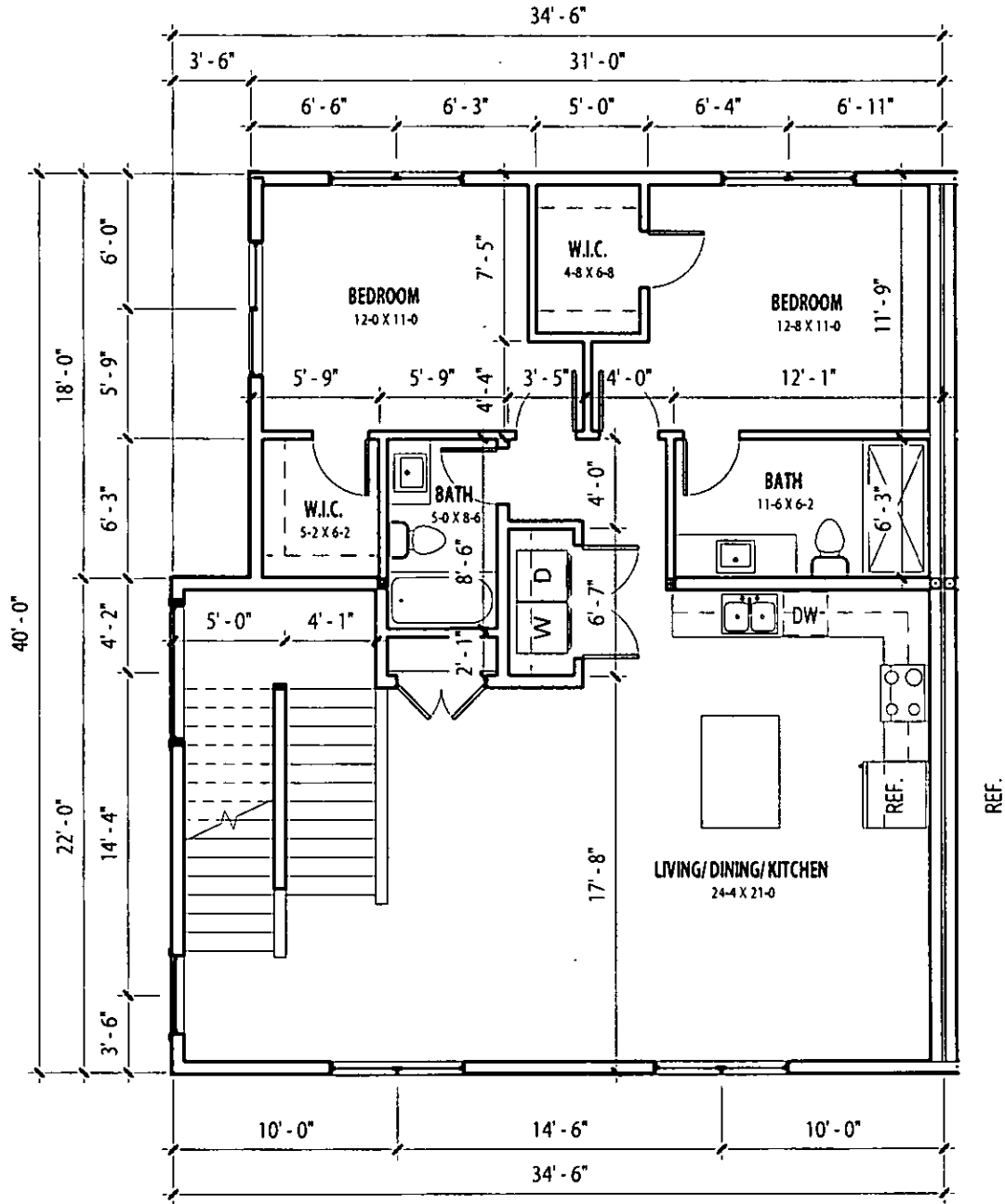
① 2ND FLOOR PLAN 1/8" = 1'-0"
