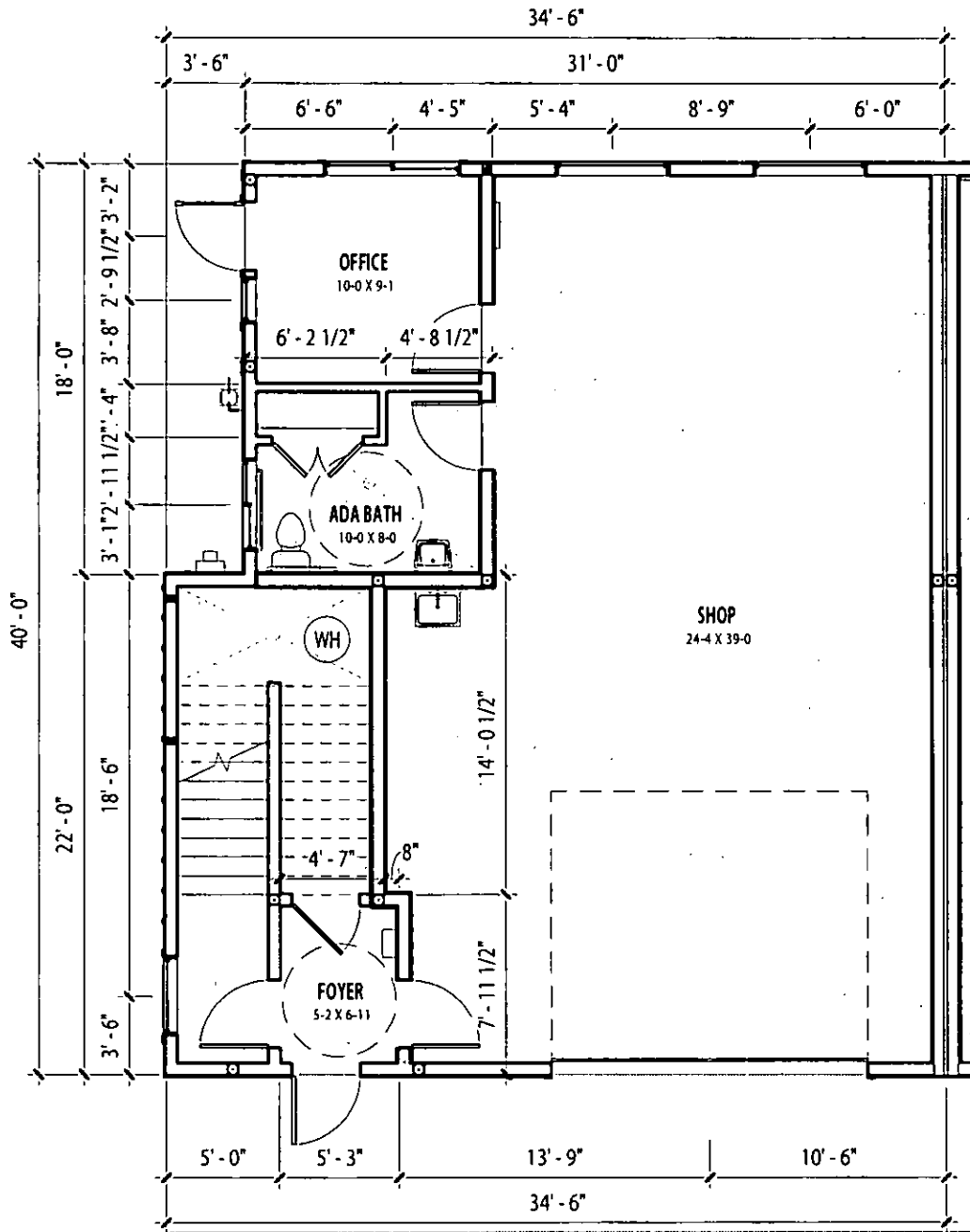
① 1ST FLOOR PLAN 1/8" = 1'-0"
