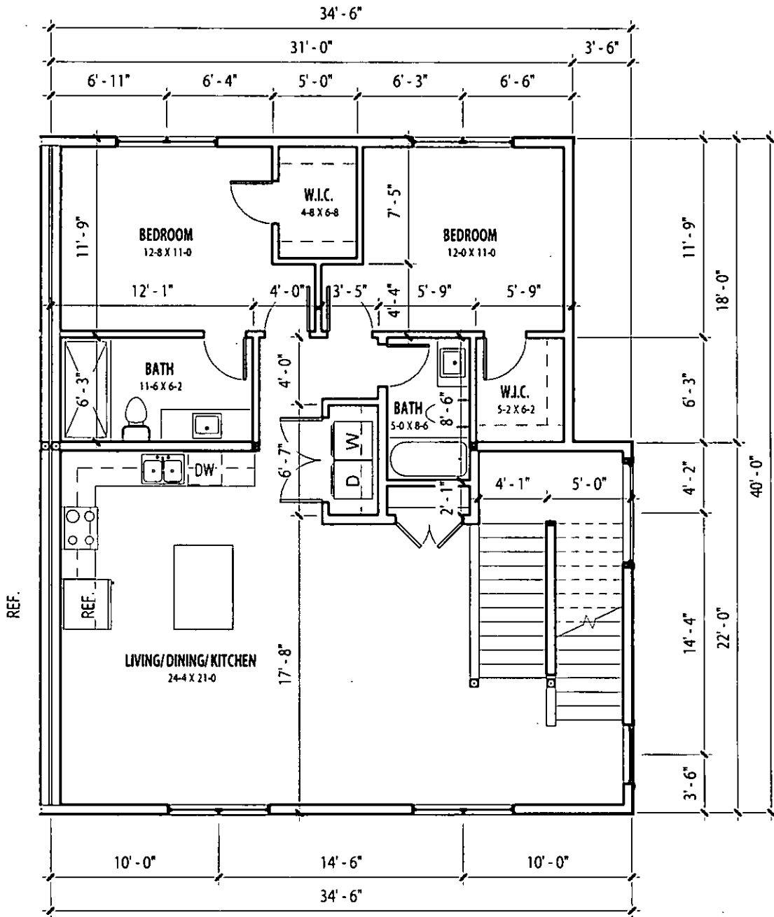
① 2ND FLOOR PLAN 1/8" = 1'-0"
