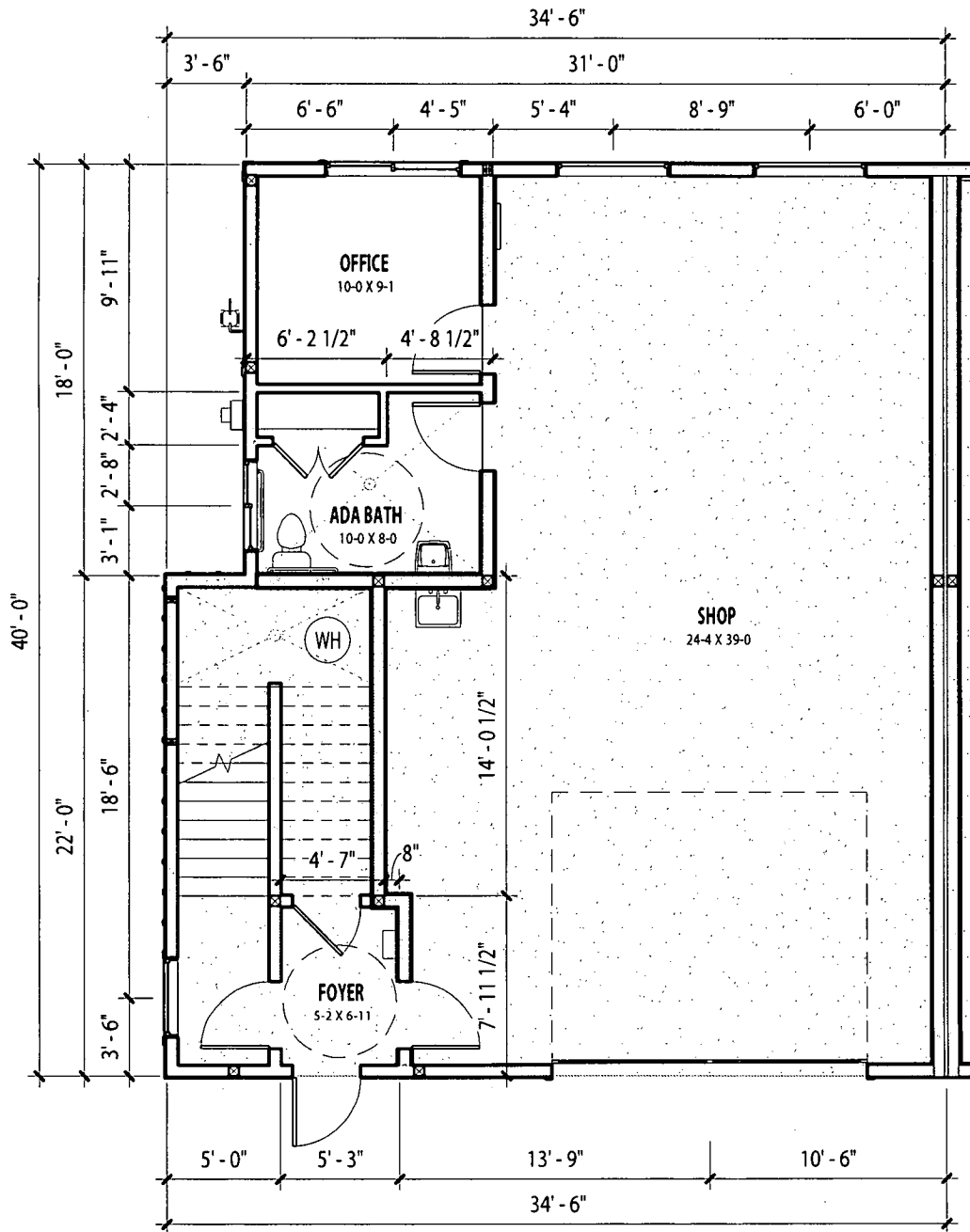
1 1ST FLOOR PLAN 1/8" = 1'-0"
