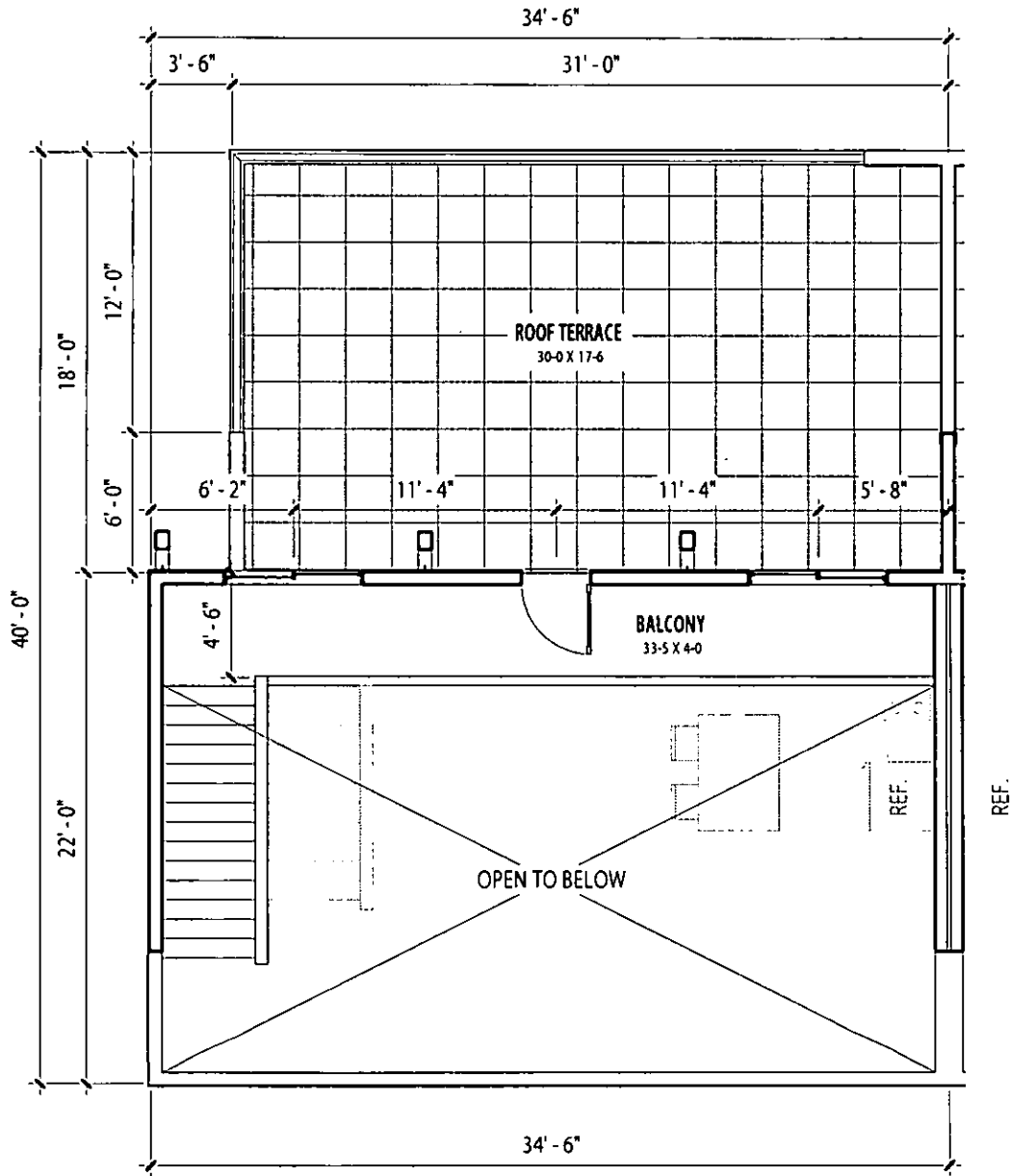
① TERRACE LEVEL 1/8" = 1'-0"
