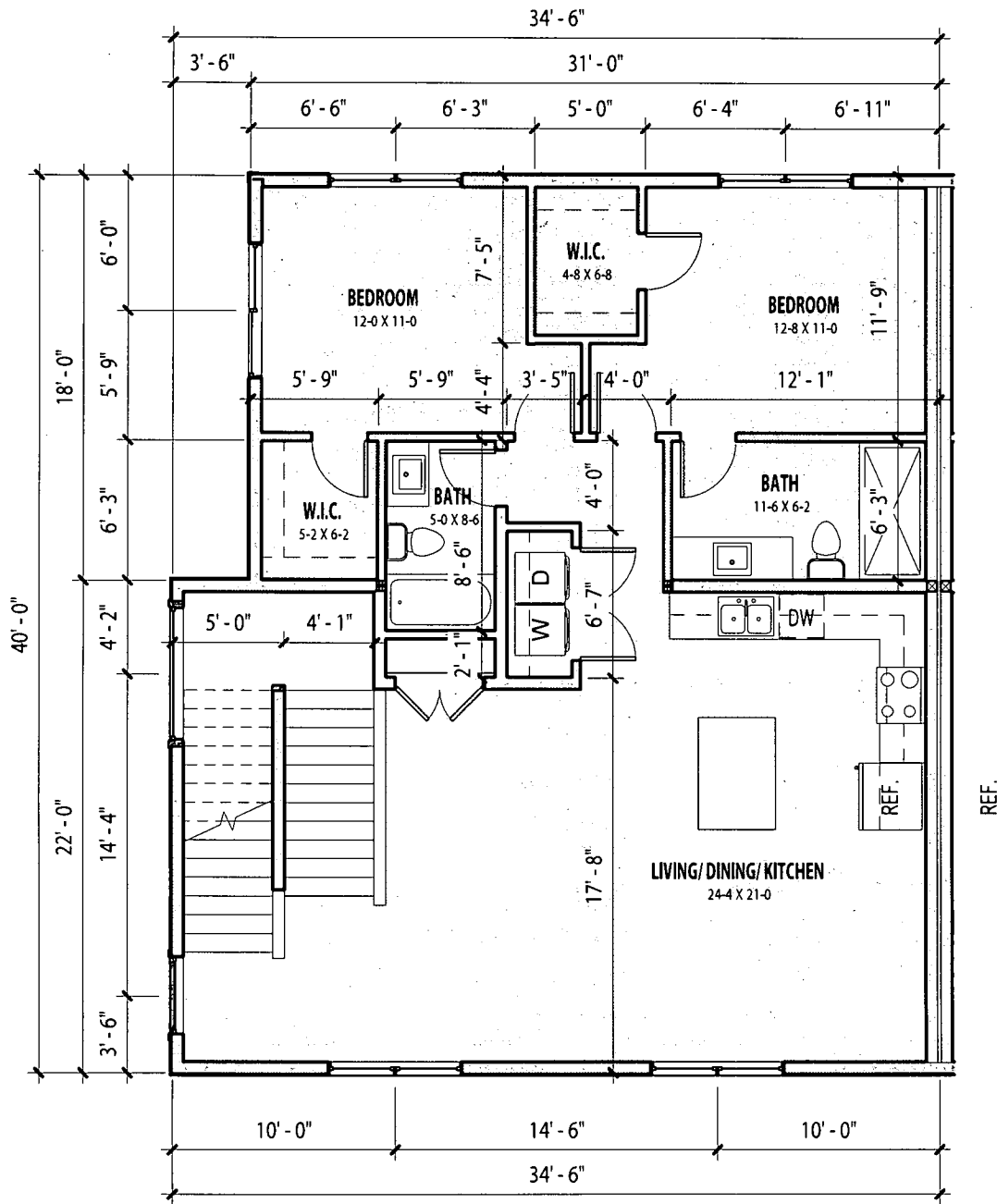
1 2ND FLOOR PLAN 1/8" = 1'-0"
